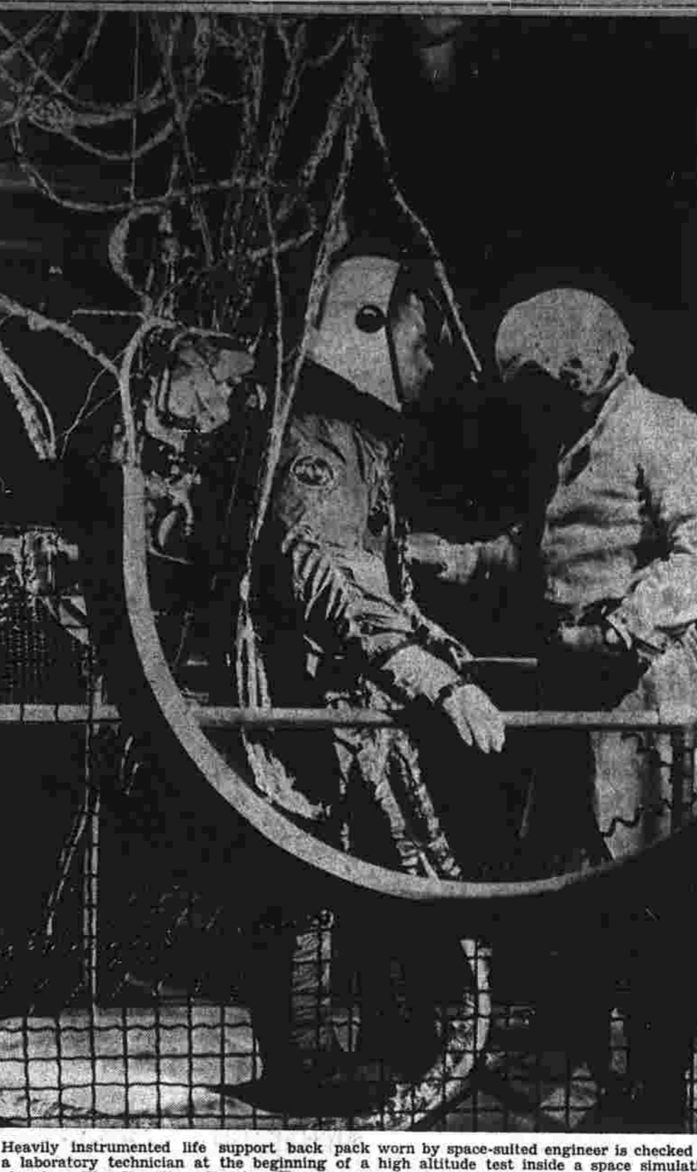
Heavily instrumented life support pack worn by space-suited engineer is checked by a laboratory technician at the beginning of a high altitude test in a space simulation chamber. The Hamilton Standard division of United Aircraft Corporation is developing the portable life support systems for the National Aeronautics and Space Administration's moonbound astronauts.
