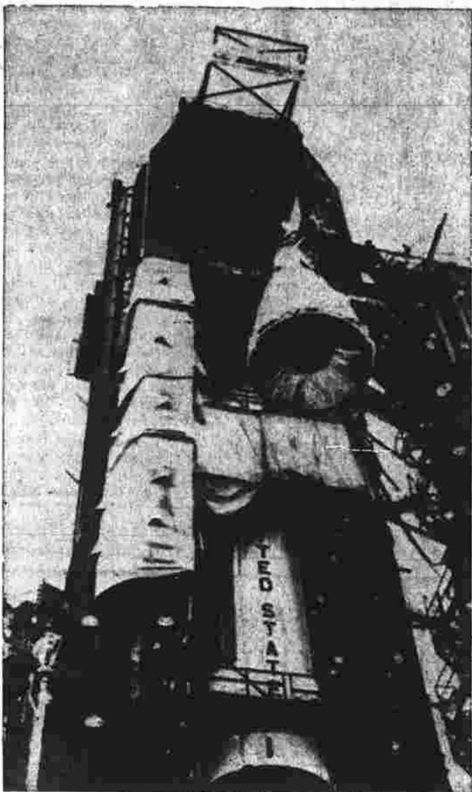
Gemini 6 spacecraft is raised into place atop Titan II rocket as technicians at Cape Kennedy speed up work for launching a week from today. Rendezvous with orbiting Gemini 7 is scheduled Dec. 14.
